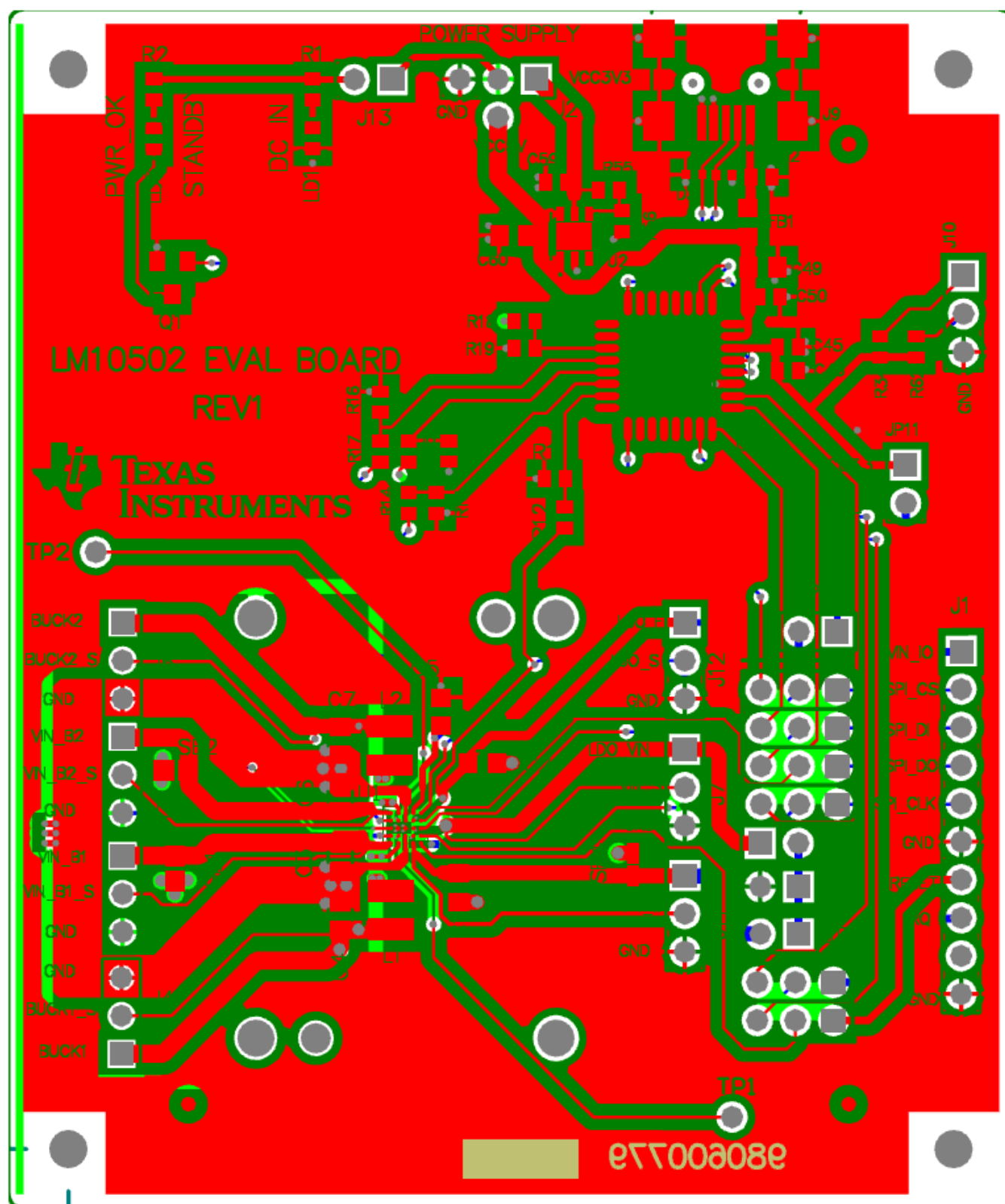
Figure 6. LM10502 Board Top Layer
